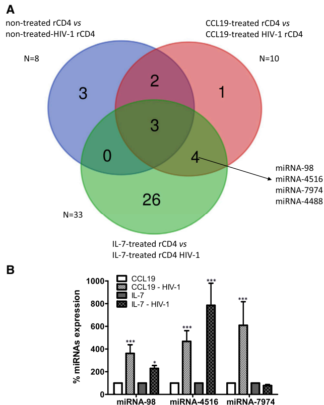
Figure 2. Differentially Expressed miRNAs Are Shared by Both CCL19- and IL-7-Based HIV-1 Latency Models
